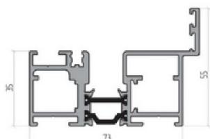
AYPCJ3F73.0201 Sim Sash (55 mm)
