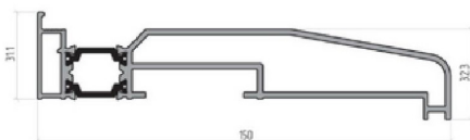
AYPC.BF73.0301 Sash transom
