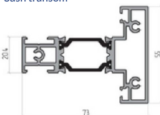
AYPC.BF73.0301 Sash transom
